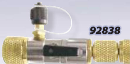
92838 Valve Core Removal Tool with Extractor Rod and 1/4" Side Port Fitting
